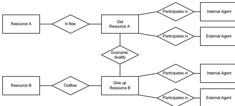
Gambar 8. Model REA
